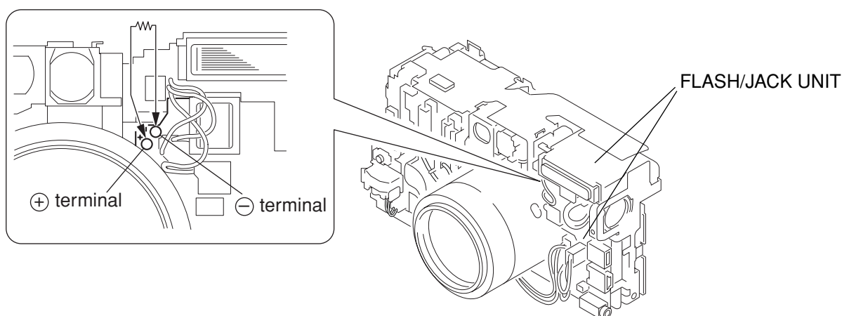
Fig. 3-1 Precaution on flash high tension circuit
