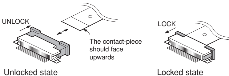
Fig. 3-2 Flexible connectors
