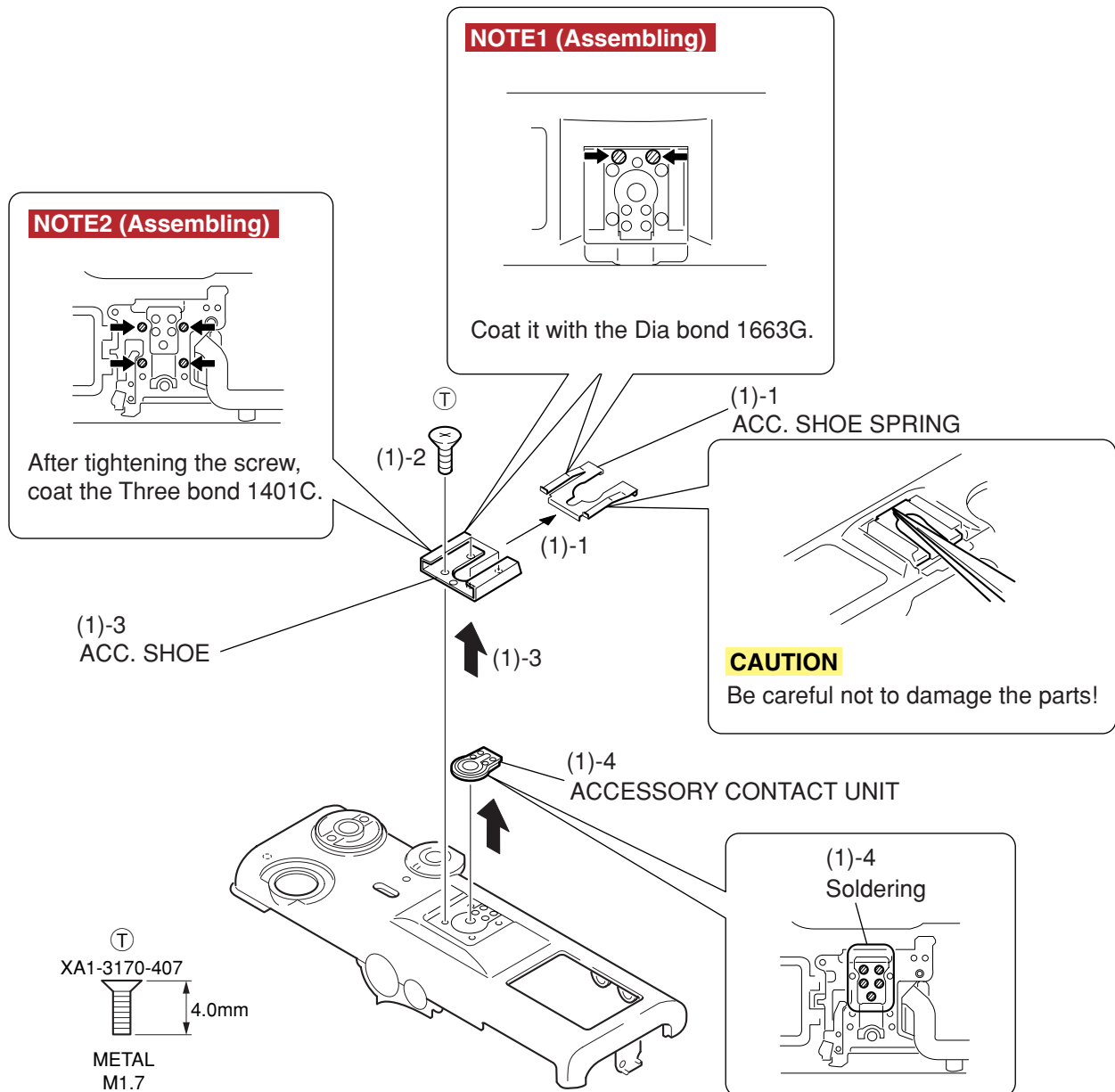
Fig. 3-23 ACCESSORY CONTACT UNIT
