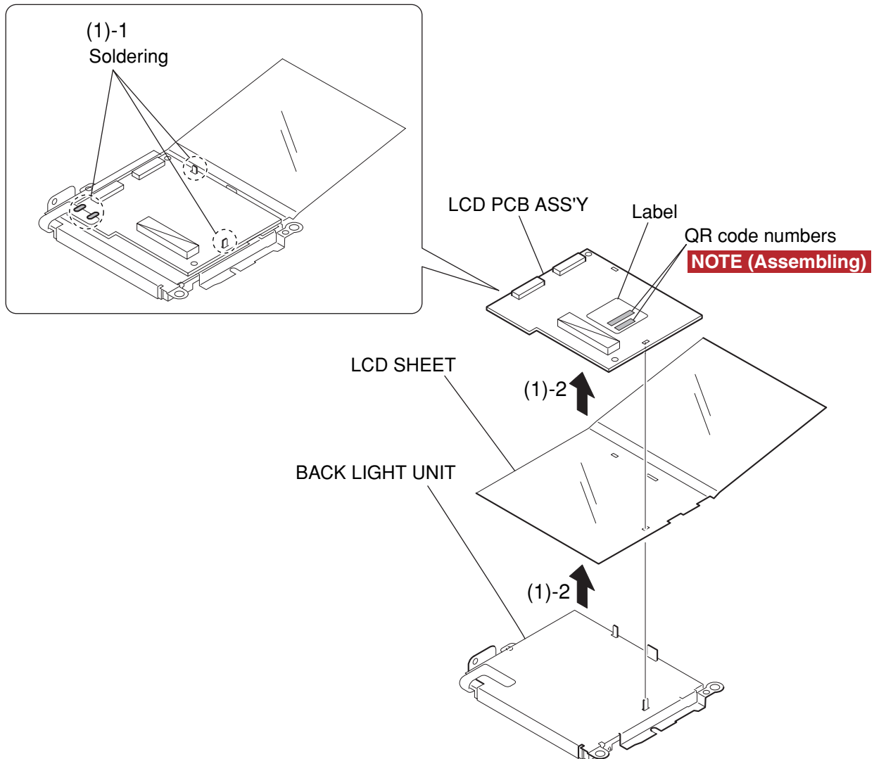
Fig. 3-26 LCD PCB ASS'Y
