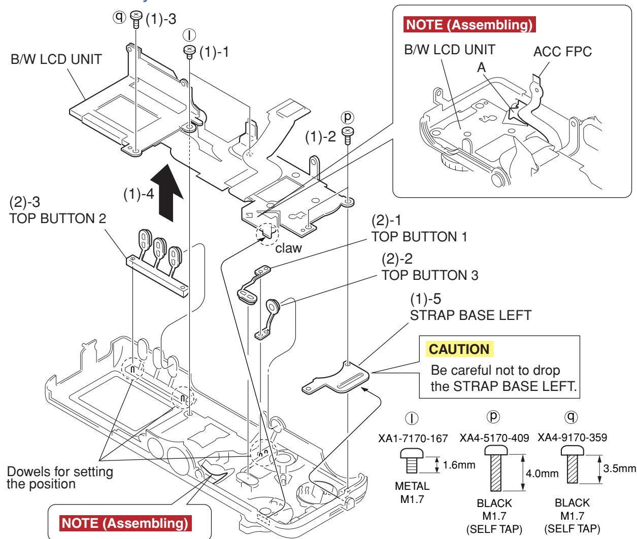
Fig. 3-19 B/W LCD UNIT, TOP BUTTON 1, TOP BUTTON 2, TOP BUTTON 3
