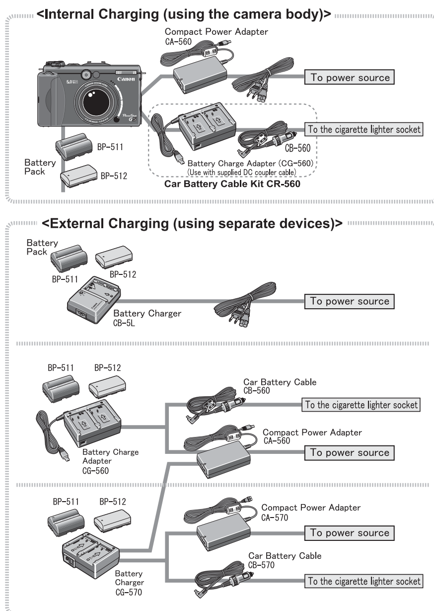
Fig. 2-2 Battery Charging System
