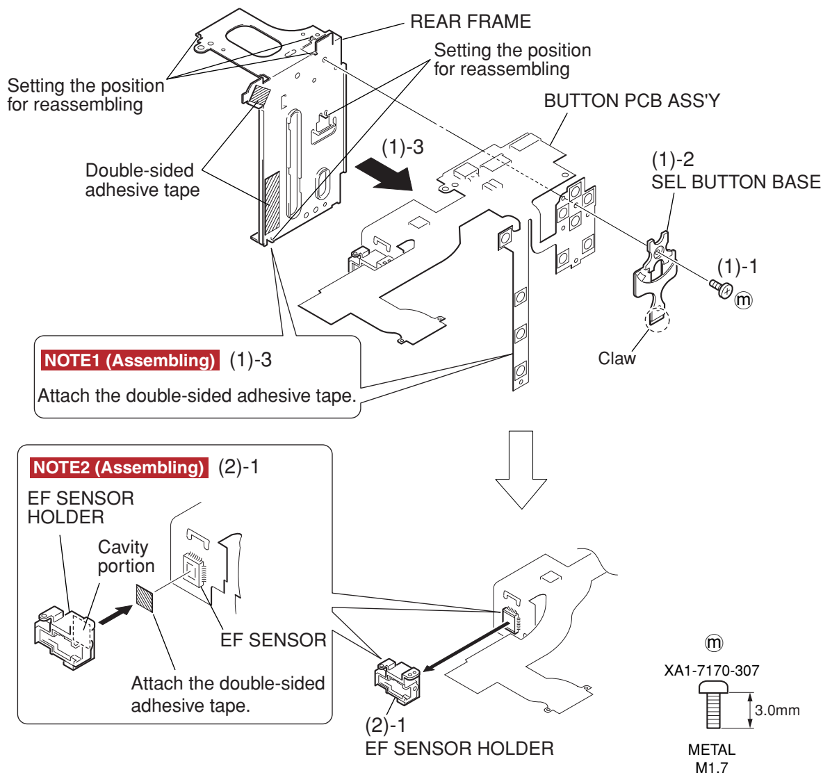
Fig. 3-27 BUTTON PCB ASS'Y, EF SENSOR HOLDER
