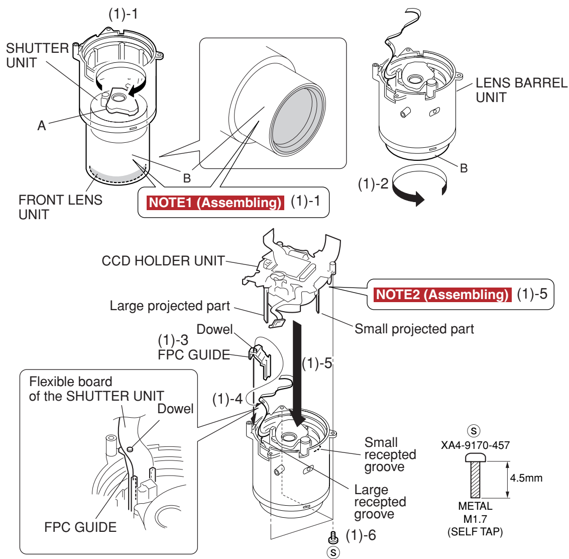
Fig.3-30 Assembling the CCD HOLDER,SHUTTER UNIT-2
